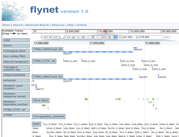
Figure 1: A snapshot of flynet JBrowse genome browser showing small peaks for the insulator CTCF (Illumina platform) and regions of histone modification H3K27me3 (Embryo stage E0-4 and S2 cells). JBrowse allows for faster and smoother navigation through the genome without requiring the reloading of the page. The annotation tracks in the left panel could be dynamically added and removed by dragging.
